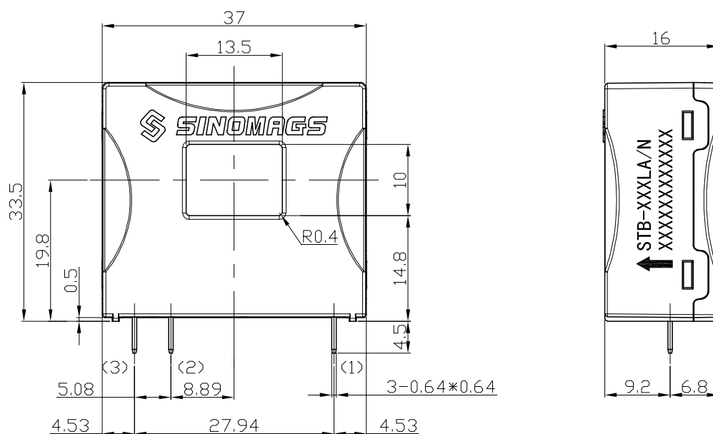
Terminals
