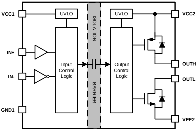
Figure 2. SiLM5350S/R/H Functional Block Diagram
