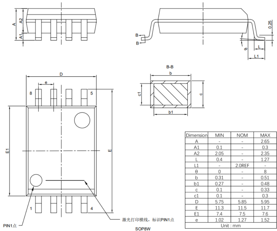
Figure 37. SOP8W Package Outline Dimensions
