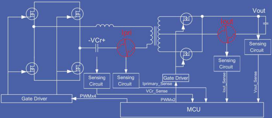
Application Schematics
