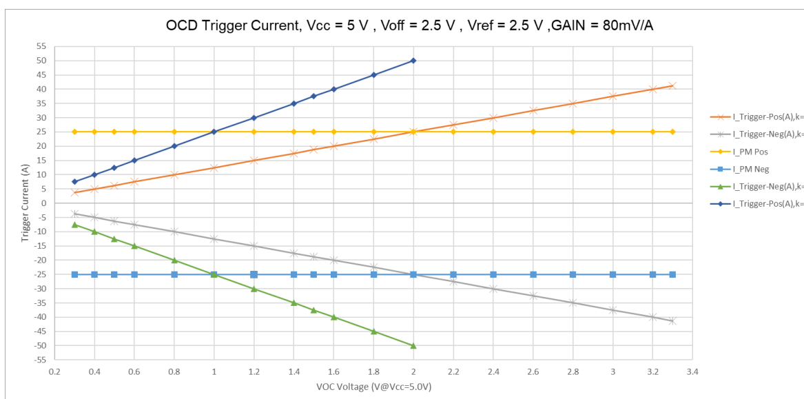
Figure 8 the relationship of trigger current and VOC setting for the STK-616A-25ML5B5, with V_{cc} = 5\text{ V} . I_{\text{trigger\_pos}} represents the forward over-current protection trigger current. I_{\text{trigger\_neg}} represents the
