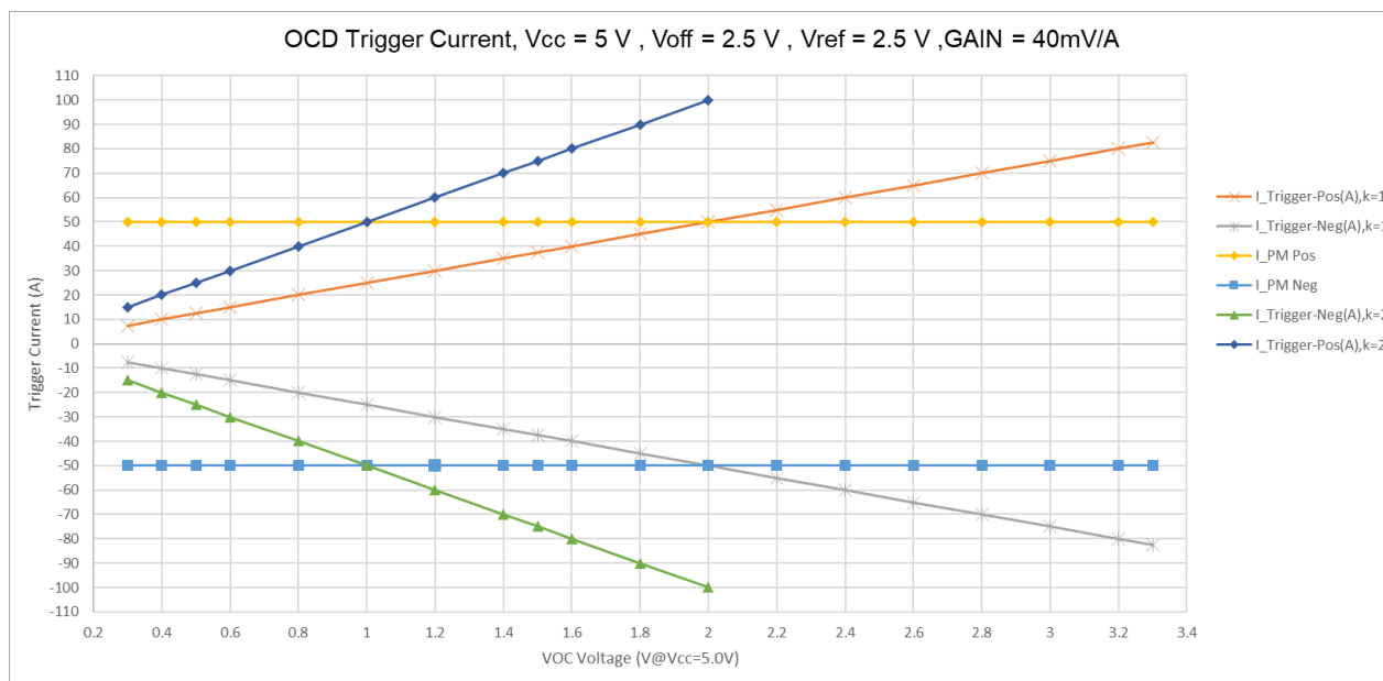
Figure 8 the relationship of trigger current and VOC setting for the STK-616T-50MLB5, with V_{cc} = 5\text{ V} . I_{\text{trigger\_pos}} represents the forward over-current protection trigger current. I_{\text{trigger\_neg}} represents the negative over-current protection trigger current. I_{\text{PN\_pos}} represents the forward primary nominal current. I_{\text{PN\_neg}} represents the negative primary nominal current. K is OCD coefficient, with typical
