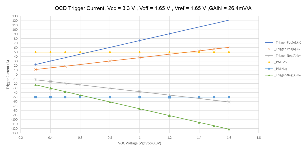
Figure 9 the relationship of trigger current and VOC setting for the STK-616T-50MLB3, with V_{cc} = 3.3\text{ V} . I_{\text{trigger\_pos}} represents the forward over-current protection trigger current. I_{\text{trigger\_neg}} represents the negative over-current protection trigger current. I_{\text{PN\_pos}} represents the forward primary nominal current. I_{\text{PN\_neg}} represents the negative primary nominal current. K is OCD coefficient, with typical values of 1, 2. I_{\text{PN}} is shown in the electrical data table.
