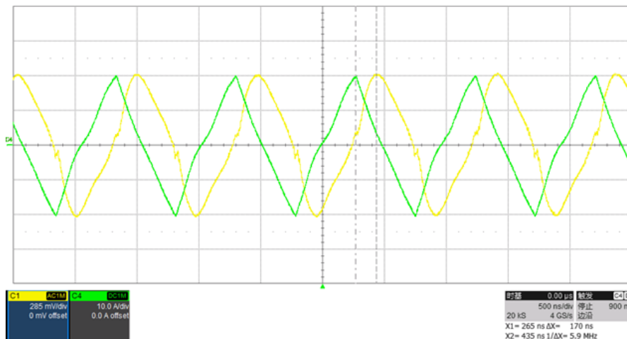
1 MHz Triangular delay---0.2 \mu s
