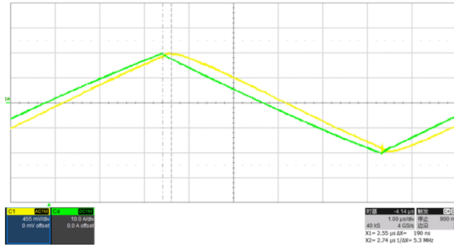
100 kHz Triangular delay---0.2 \mu s
